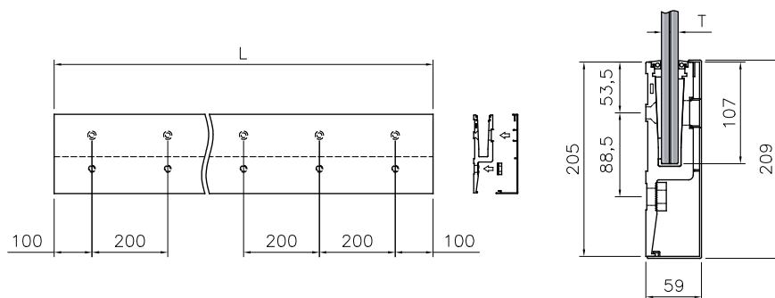
Floor profile Horizon “Y” - profile including cover
