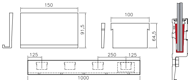
Set of locking wedges for 1 mt of Horizon “Y”
